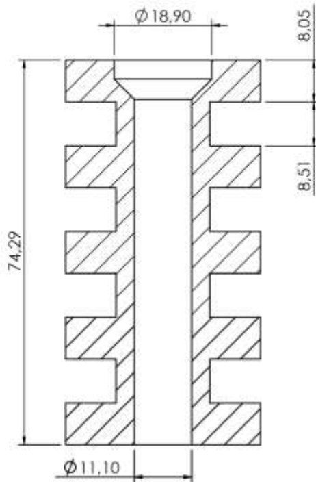
SECTION E-E
